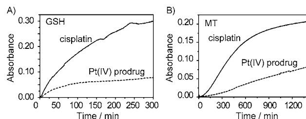
Figure 6. Time course of reactions of platinum complexes with GSH or MT at 37°C, pH 7.0. A) Reaction of GSH (16 mM) with cisplatin (32 μM, solid line) and the platinum(IV) prodrug ( c,c,t -[Pt(NH 3 ) 2 Cl 2 (O 2 CCH 2 CH 2 CO 2 H) 2 ]; 32 μM, dashed line). B) Reaction of MT (10 μM) with cisplatin (20 μM, solid line) and the platinum(IV) prodrug (20 μM, dashed line). Reactions were monitored by observing the increase in the absorption at 260 nm for the GSH reaction (A) and at 285 nm for the MT reaction (B).
